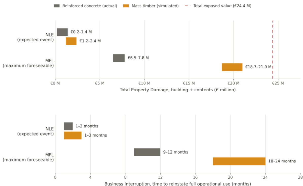
Graph 3, Ranges from the MFL and NLE scenarios (Case Study #4), applied to the provisional building replacement value of €20M and to the insured contents value of €4.4 M. Durations and percentages exclude temporary relocation costs
