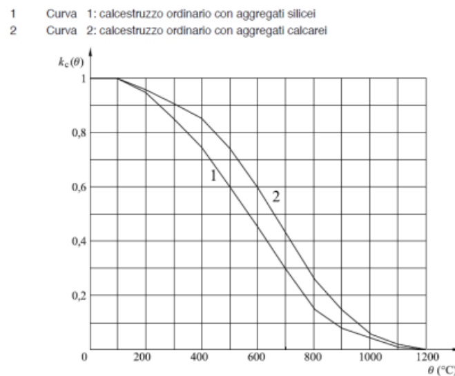
Fig. 3, Trend of the coeff. k_c(\theta) as a function of temperature \theta (EN 1992-1-2:2005)
