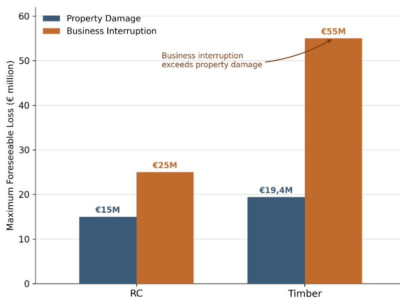
Graph 2, Property Damage and Business Interruption under the MFL scenario, Case Study #1
