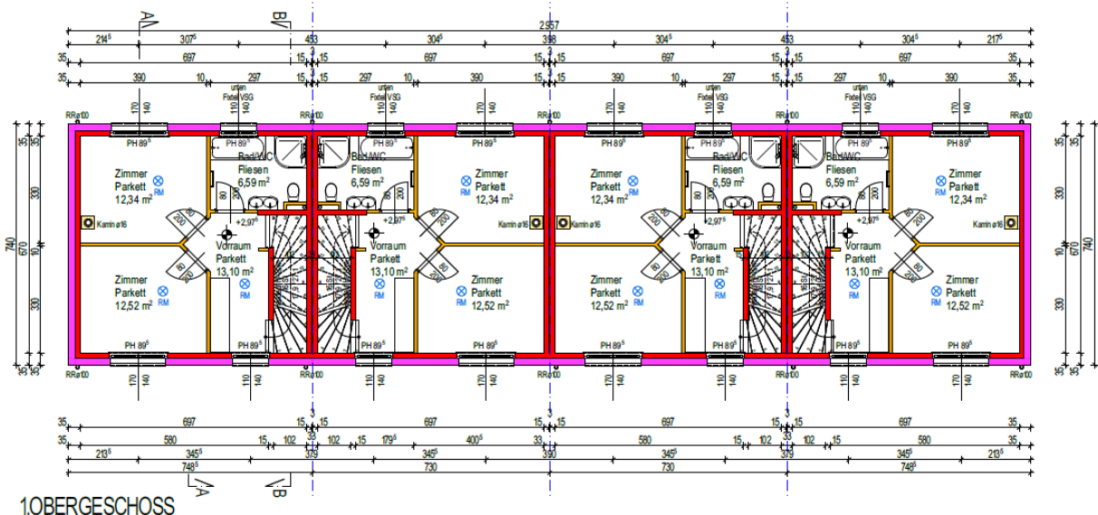
Fig. 13, Detail of the first floor
