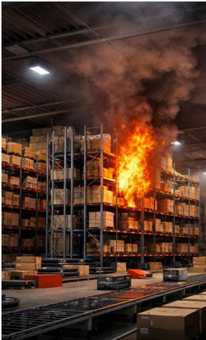
Fig. 10, Simulated image of an early stage of the fire under MFL conditions
