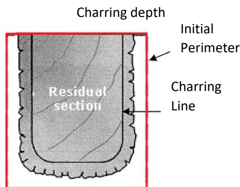
Fig. 6, Charring behaviour and Effective Cross Section
