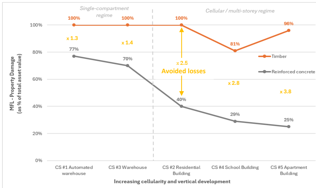
Graph 4, MFL: timber versus reinforced concrete across the five case studies
