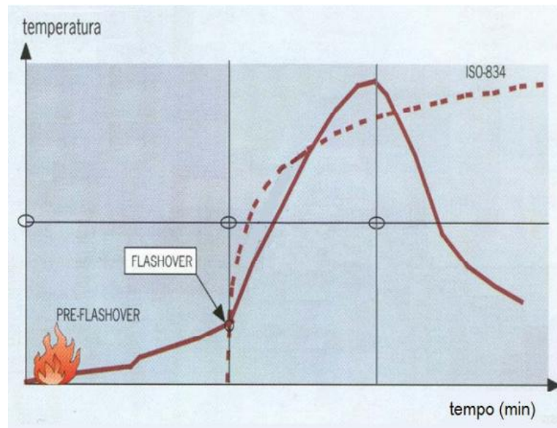
Fig. 7, Natural fire curves compared with the ISO 834 standard fire curve (Ing. G. Biffarella, 2014)
