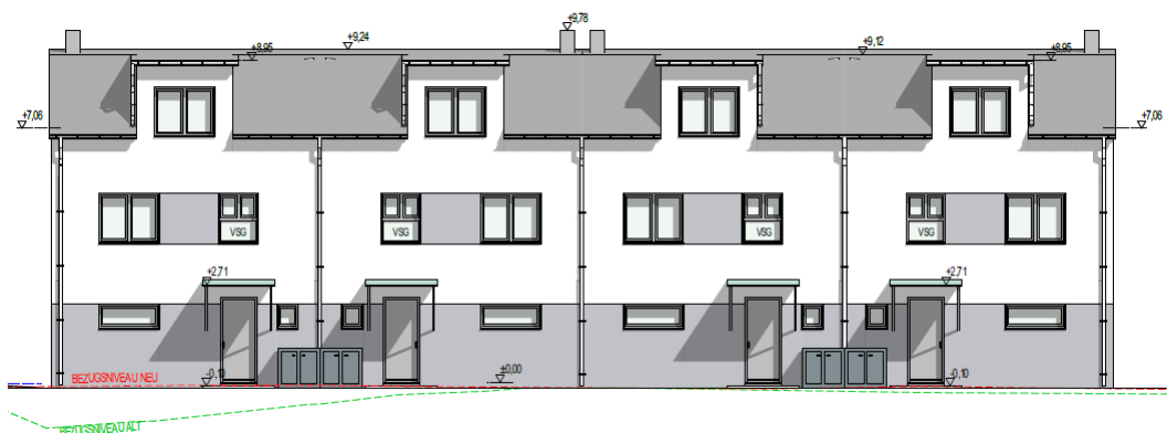
Fig. 12, View of the entrance facade
